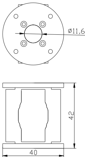
K/Ka band circular polarizer (type B)
