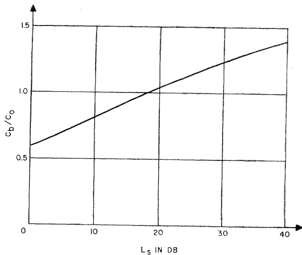
Fig. 4—Beamwidth of a Dolph-Tchebycheff array vs sidelobe level L_S relative to a uniformly illuminated array of equal aperture.
