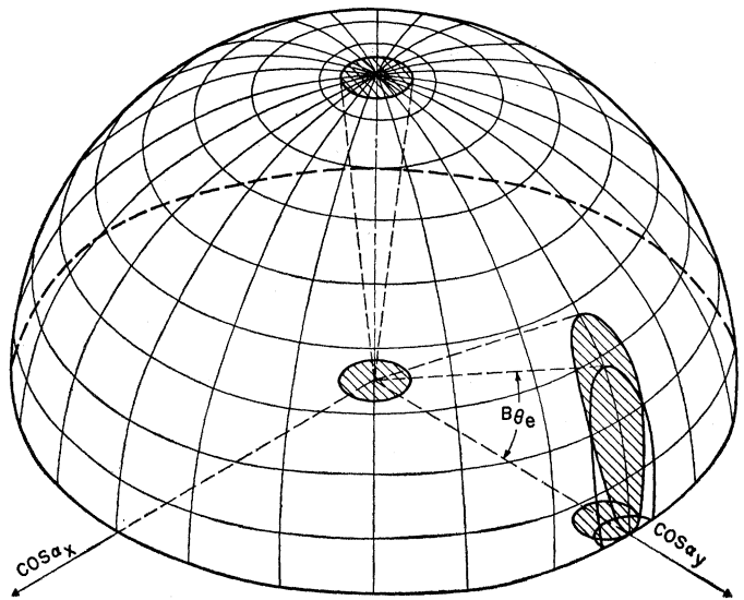
Fig. 10—Beam approaching endfire position.
