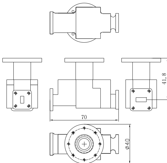
K/Ka band different frequency OMT
