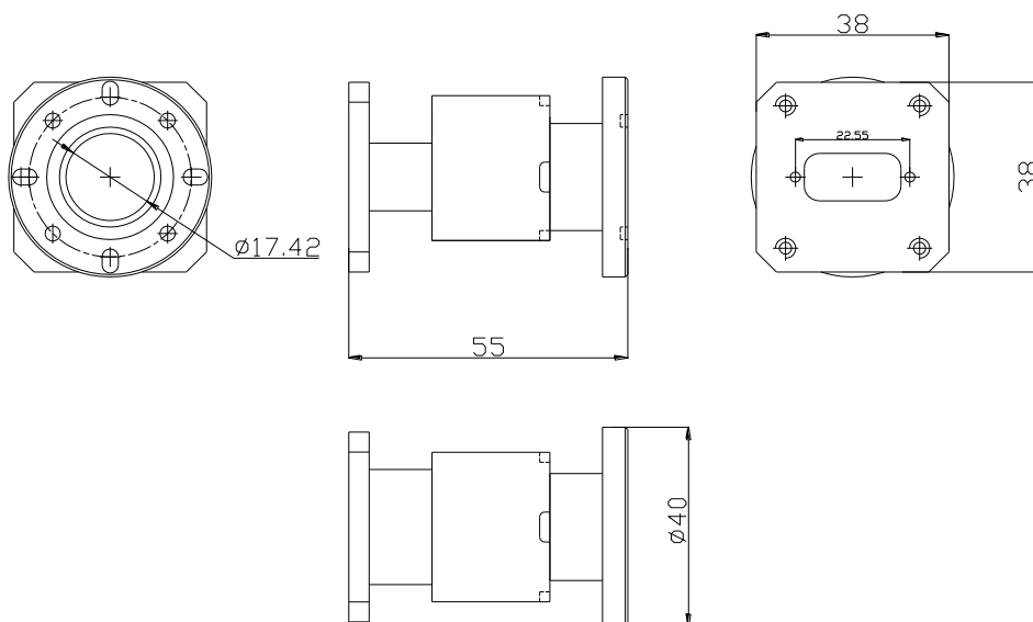
Ku band absorptive OMT
