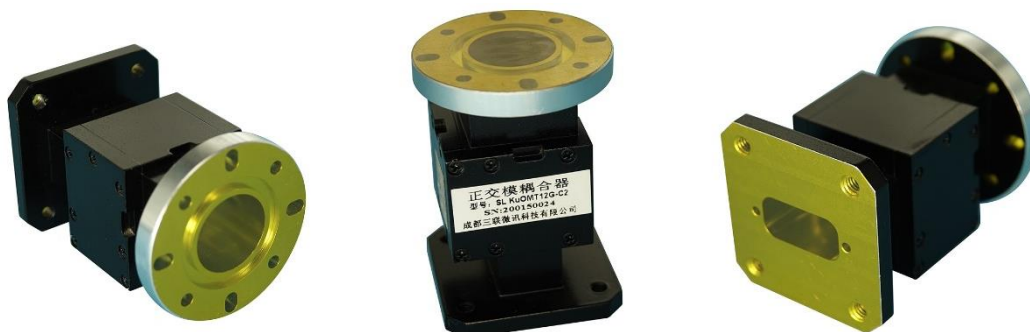
Ku band absorptive OMT
