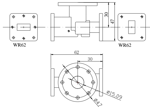
Ku Band same frequency inphase OMT(type D)
