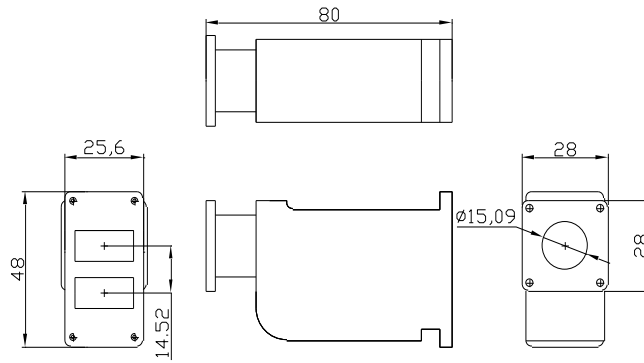
Ku Band same frequency inphase OMT(type C)
