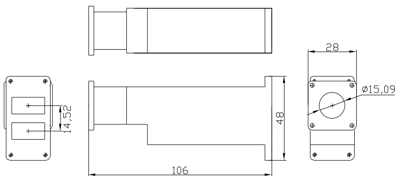
Ku Band same frequency inphase OMT(type B)
