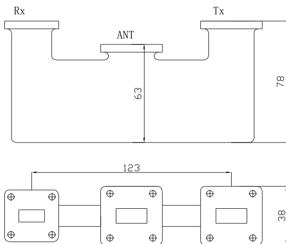
Ku Band Satellite Communication Duplexer (Type C)
