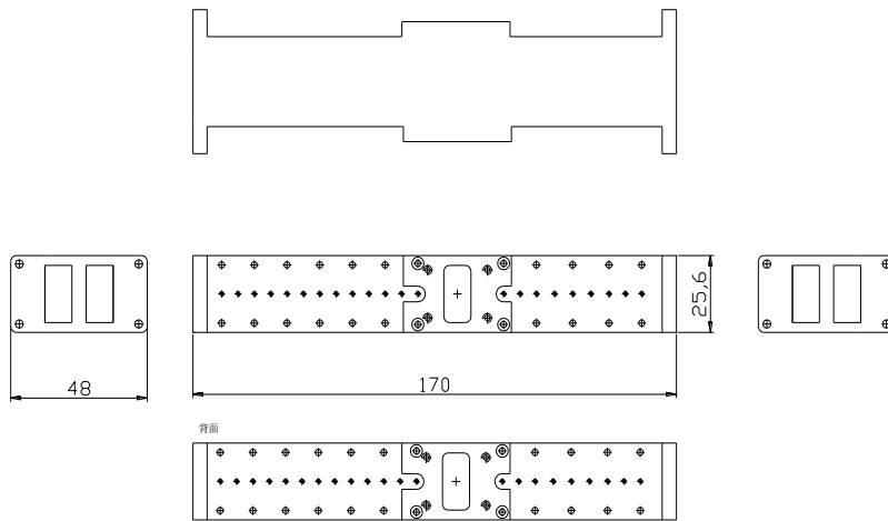
Ku Band Satellite Communication Duplexer
